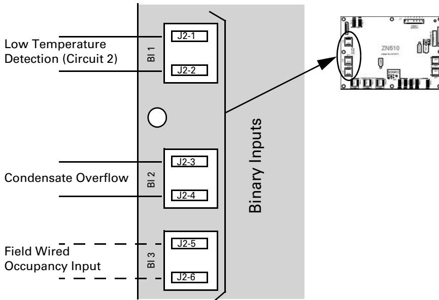
Figure 6: Binary inputs.
