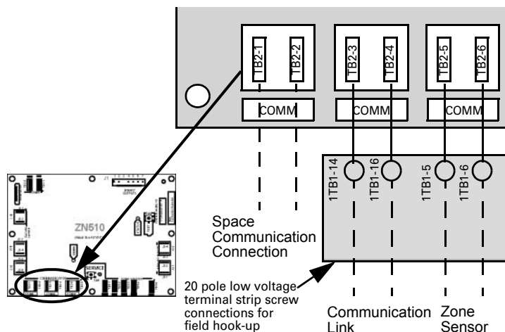
Figure 3: Communication Wiring
